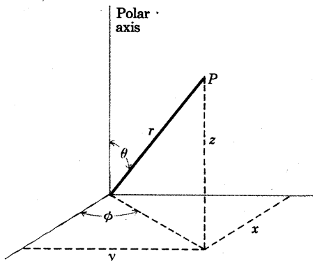
Fig. 12 The relation between rectangular and spherical polar coordinates of a point P .
