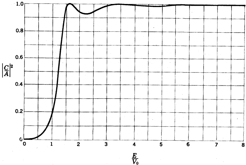
Fig. 15 The transmission coefficient of a square barrier as a function of particle energy for mV_0a^2/\hbar^2 = 8 .
