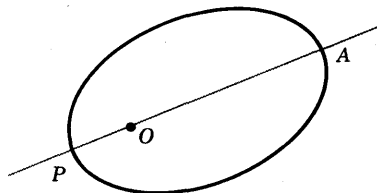
Fig. 25 Classical Kepler orbit with the center of attraction at a focus O of the ellipse.
