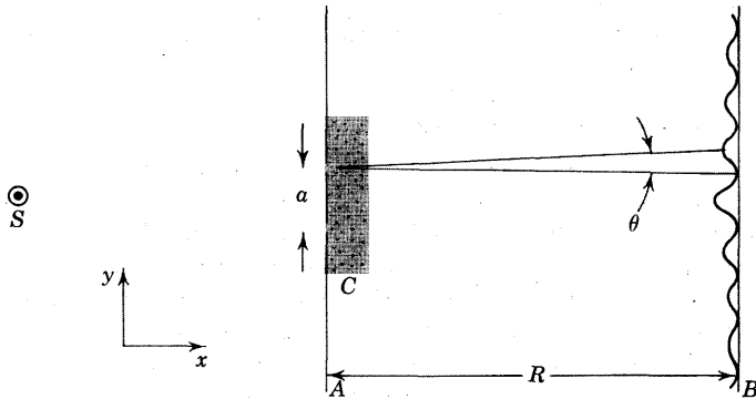
Fig. 3 The experimental arrangement of Fig. 1, modified by the addition of photon indicators C .
