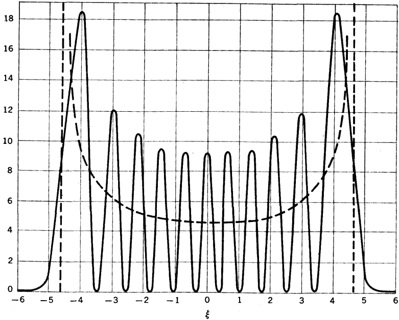
Fig. 11 The position probability density for the state n = 10 of a harmonic oscillator (solid curve) and for a classical oscillator of the same total energy (dashed curve). [After L. Pauling and E. B. Wilson, Jr., "Introduction to Quantum Mechanics," p. 76 (McGraw-Hill, New York, 1935).]
