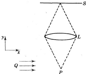
Fig. 2 An experiment for the localization of a particle P by means of one of the scattered quanta Q , which is focused by the lens L to form an image on the screen S .
