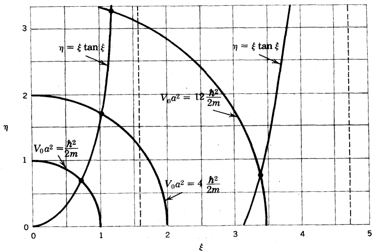
Fig. 8 Graphical solution of Eq. (9.7) for three values of V_0a^2 ; the vertical dashed lines are the first two asymptotes of \eta = \xi \tan \xi .
