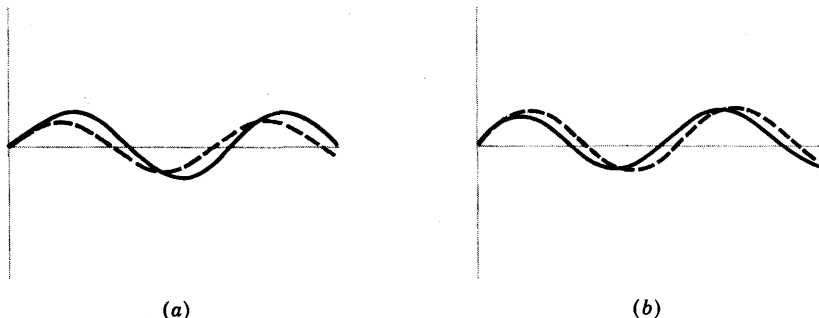
Fig. 22 Graphs of the effects of (a) positive (repulsive) potential and (b) negative (attractive) potential on the force-free radial wave function rj_0(kr) (dotted curves). The solid curves are \chi_0(r) . (Graphs supplied by J. L. Schwartz and H. M. Schey.)
