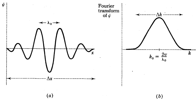
Fig. 4 Plots of a typical wave packet \psi(x) and its Fourier transform.
