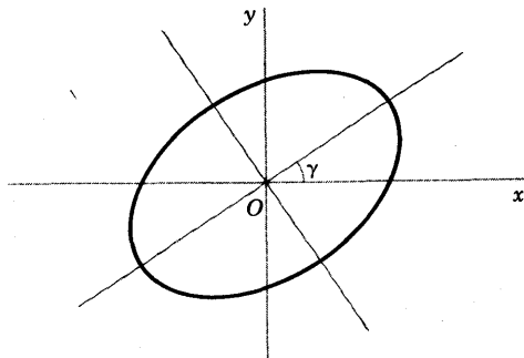
Fig. 26 Classical harmonic-oscillator orbit with the center of attraction at the center O of the ellipse.
