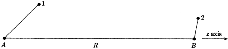
Fig. 27 Two hydrogen atoms, with nuclei at A and B separated by a distance R , have electrons at 1 and 2; their interaction is given by H' in Eq. (32.11).
