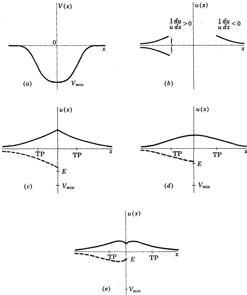
Fig. 5 (a) Potential-energy function and (b) solutions for large |x| ; (c) and (e) show that either the wave function or its slope is discontinuous at x = 0 for values of E that are smaller (more negative) and larger, respectively, than the energy eigenvalue shown in (d).
