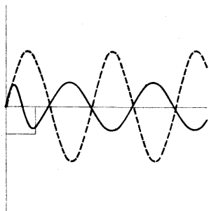
Fig. 23 Graphs of rj_0(kr) (dotted curve) and \chi_0(r) (solid curve) when the attractive square well potential is strong enough to make \delta_0 = 180^\circ . The two wave functions start out with the same slope at r = 0 , and \chi_0(r) is pulled in by half a cycle. (Graphs supplied by J. L. Schwartz and H. M. Schey.)
