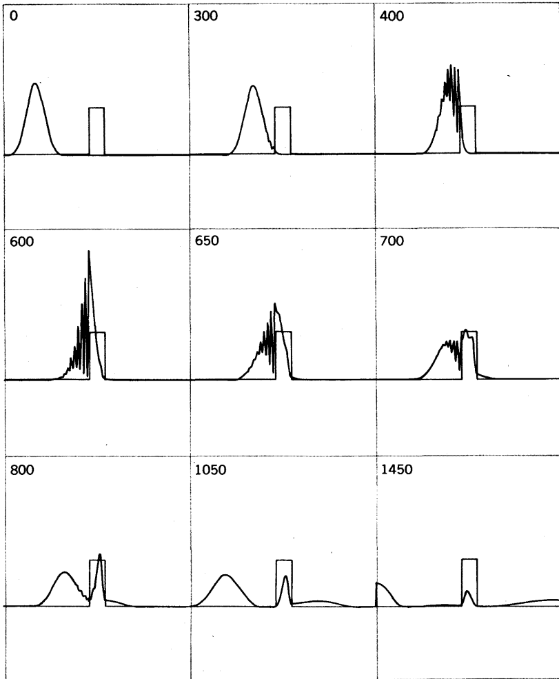
Fig. 17 Same as Fig. 16, with the mean energy equal to the barrier height.
