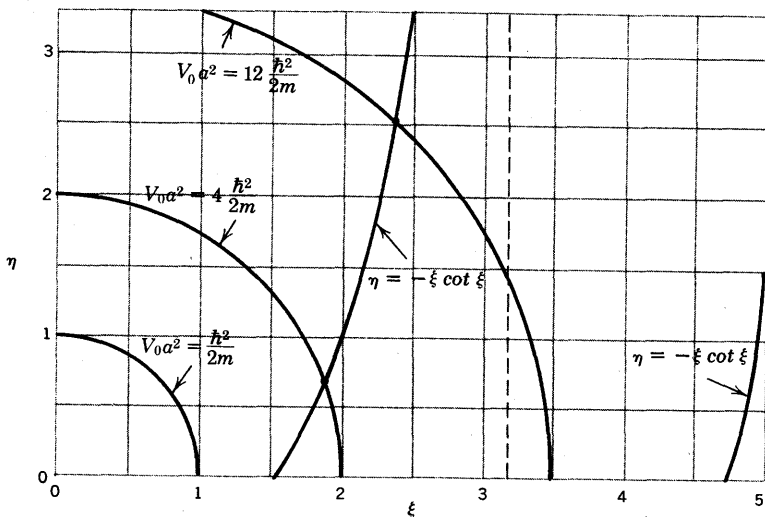
Fig. 9 Graphical solution of Eq. (9.6) for three values of V_0 a^2 ; the vertical dashed line is the first asymptote of \eta = -\xi \cot \xi .
