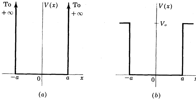
Fig. 7 One-dimensional square well potential with (a) perfectly rigid walls and (b) finite potential step.
