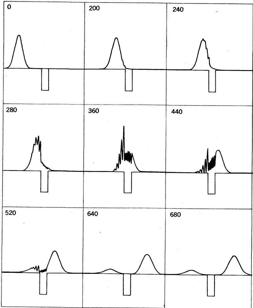
Fig. 18 Gaussian wave-packet scattering from a square well when the mean energy of the packet is half the well depth.
