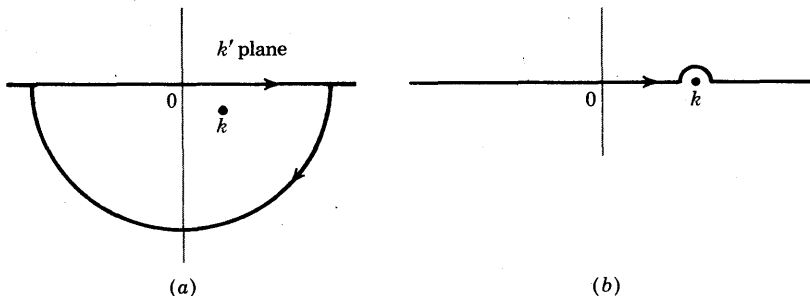
Fig. 36 Contours for the evaluation of Eq. (39.21).
