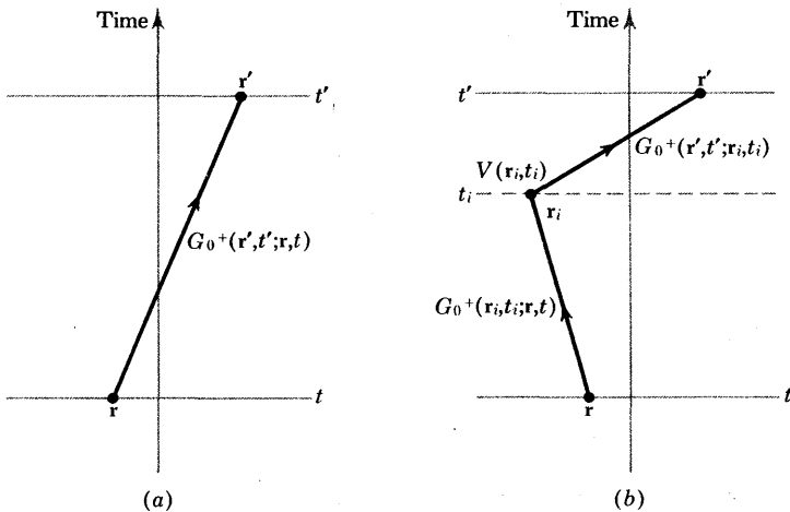
Fig. 33 Schematic representation of the first term (a) and second term (b) on the right side of Eq. (36.15).
