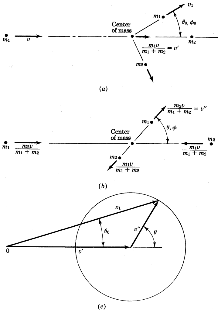
Fig. 20 (a) Laboratory coordinate system, in which the target particle of mass m_2 is initially at rest. (b) Center-of-mass coordinate system, in which the center of mass is initially and always at rest. (c) Vector addition of velocity of center of mass in laboratory system ( v' ) to velocity of observed particle in center-of-mass system ( v'' ) to give velocity observed in laboratory system ( v_1 ); if v'' < v' , \theta_0 cannot exceed the angle \sin^{-1}(v''/v') .
