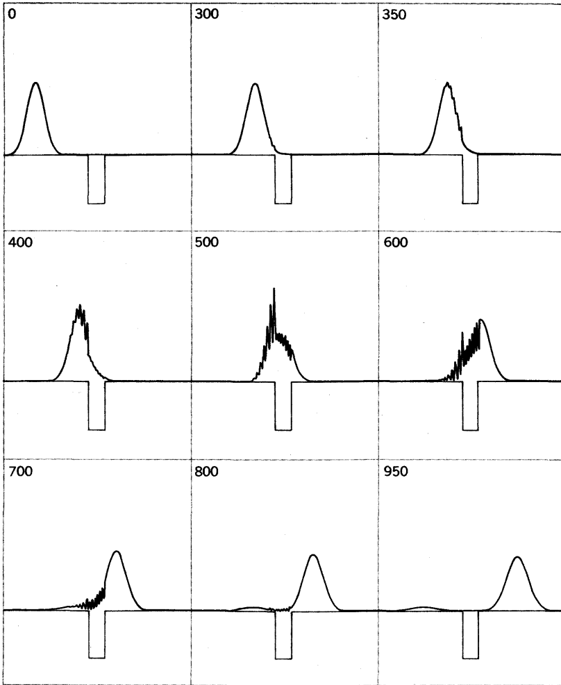
Fig. 19 Same as Fig. 18, with the mean energy equal to the well depth.
