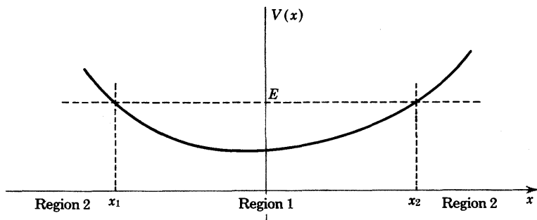
Fig. 29 Application of the WKB method to a potential trough; linear turning points occur at x_1 and x_2 .
