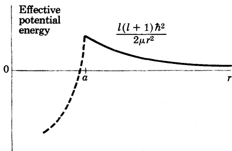
Fig. 24 The effective potential energy [V(r) \text{ plus "centrifugal potential"}] for l > 0 , when V = 0 for r > a . The dashed portion for r < a depends on the shape of V . The effective potential barrier ( r \geq a ) resembles the barrier of Fig. 14 in that it has a small transmission for E slightly greater than zero.
