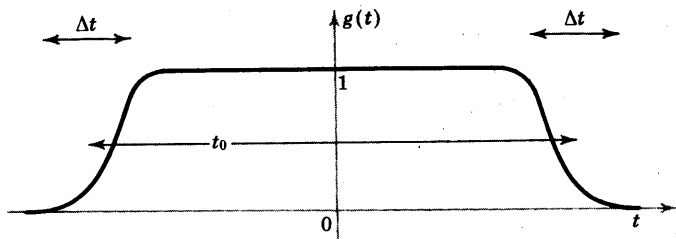
Fig. 34 Schematic plot of the function g(t) that determines the time dependence of V .
