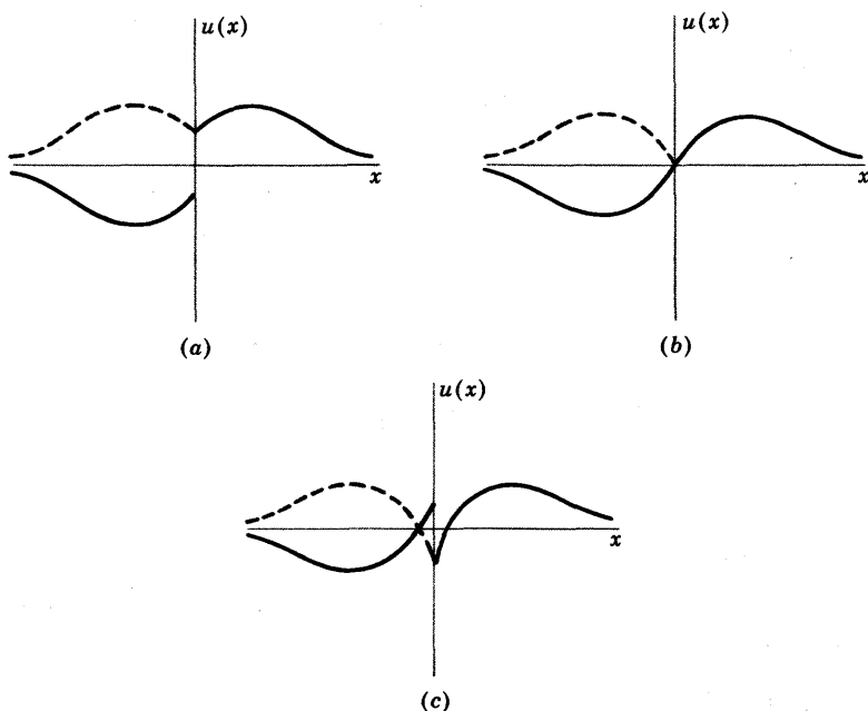
Fig. 6 Solutions for sufficiently broad or deep potential and larger (less negative) values of E than those shown in Fig. 5. E increases from (a) to (b) to (c) and is an eigenvalue in (b), where the wave function and its slope can both be continuous at x = 0 .
