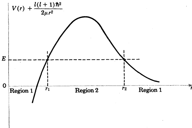
Fig. 30 Application of the WKB method to a potential barrier, with the radial coordinate as the independent variable.
