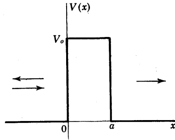
Fig. 14 A one-dimensional square potential barrier of height V_0 and thickness a .
