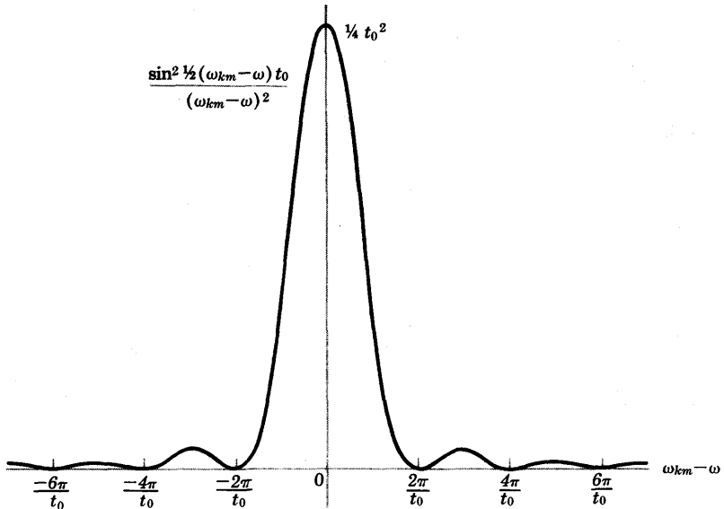
Fig. 31 The ordinate is proportional to the first-order perturbation probability of finding a system in a state of energy E_k \equiv E_m + \hbar\omega_{km} ; the heights of the secondary peaks fall off like 1/(\omega_{km} - \omega)^2 .
