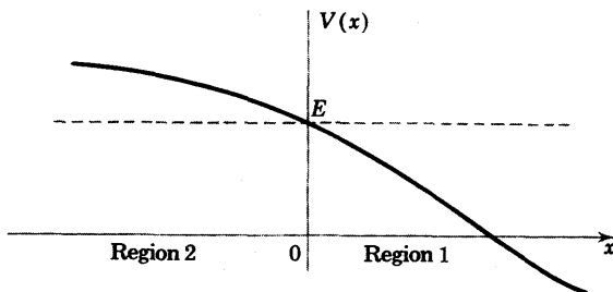
Fig. 28 A typical linear turning point, where V(x) = E at x = 0 ; in region 1, E > V(x) , and in region 2, E < V(x) .
