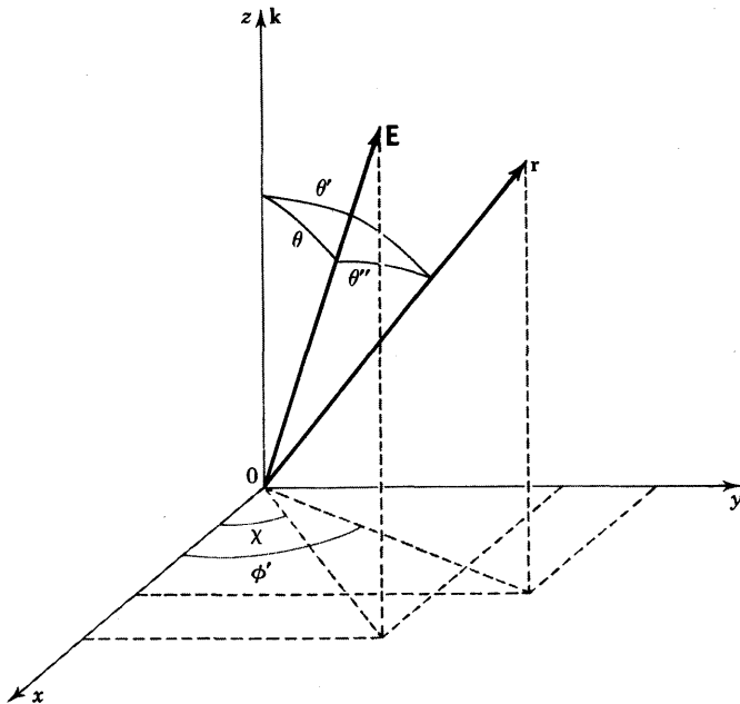
Fig. 32 Diagram for the integration of the matrix element (35.19).
