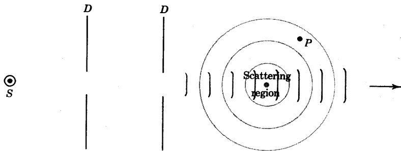
Fig. 21 Schematic diagram of a laboratory arrangement for the measurement of scattering, in which there is no interference between the incident and scattered waves at the point of observation, P .
