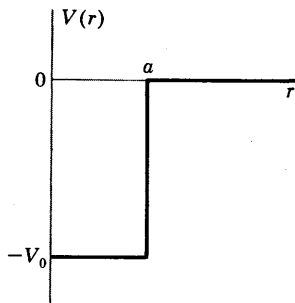
Fig. 13 A spherically symmetric square well potential of depth V_0 and radius a .
