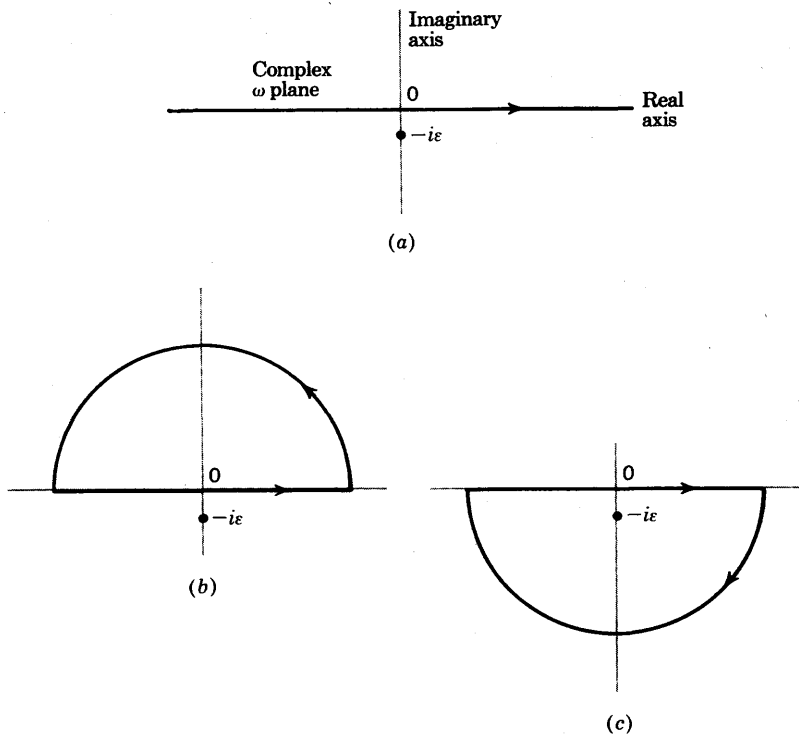
Fig. 35 Contours for the integration of Eq. (37.7).
