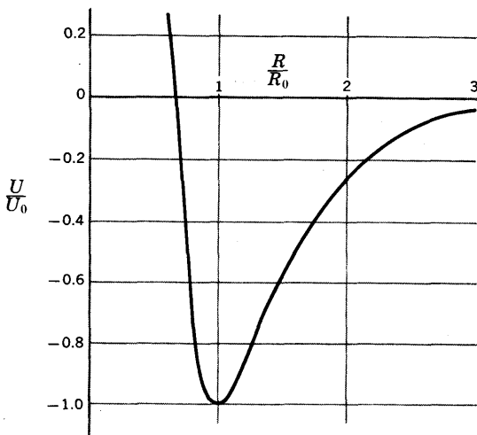
Fig. 39 The Morse potential (49.16), with a = \frac{1}{2}R_0 .
