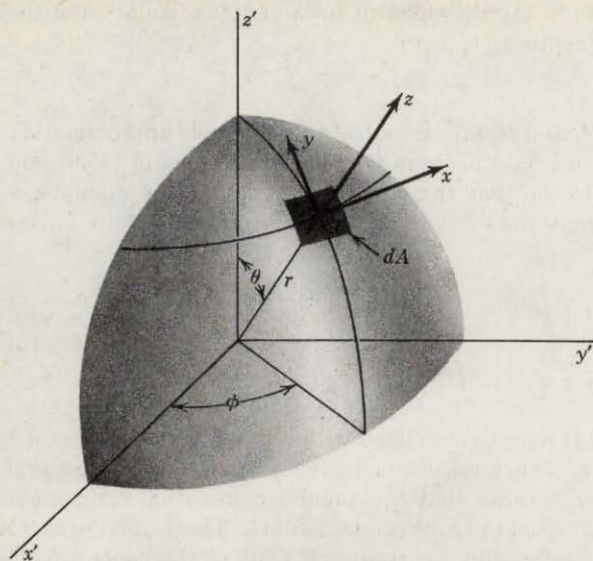
Fig. 38 The relation between the unprimed coordinate system of Eqs. (45.15) and the primed coordinate system of Eq. (45.16).
